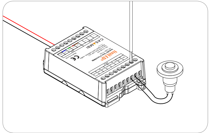
6. Optional: Connect the pushbutton(s).
