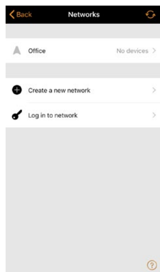
6. Select network
