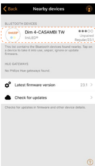
17. Select device
