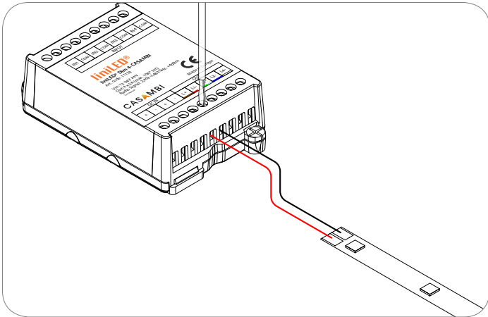
5. Connect the LED strip wires to the outputs according to the wiring scheme on page 7.
