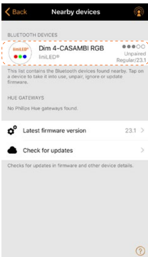
13. Select device
