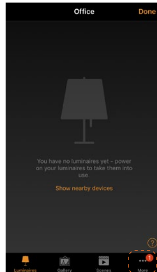
11. Select More
